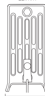
footed end section depth = 252mm
