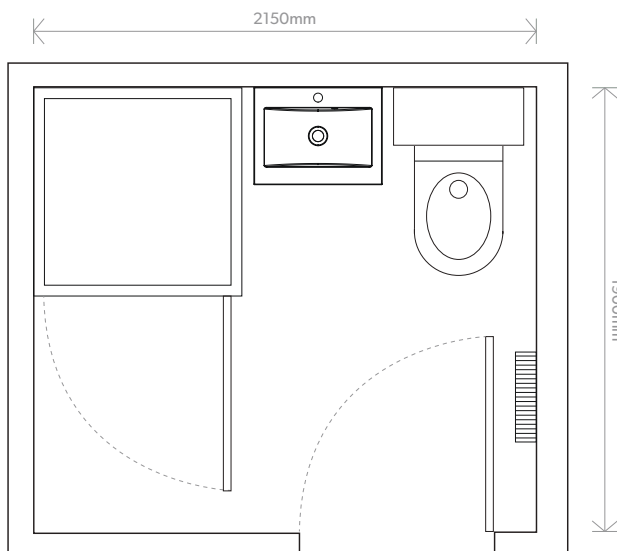
Reveal 60 Compact Wall Hung Unit
